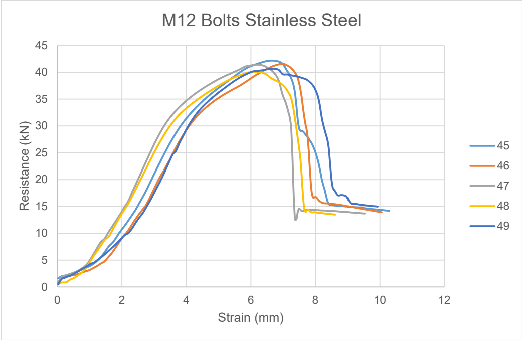
Figure A.7 M12 stainless steel test results
