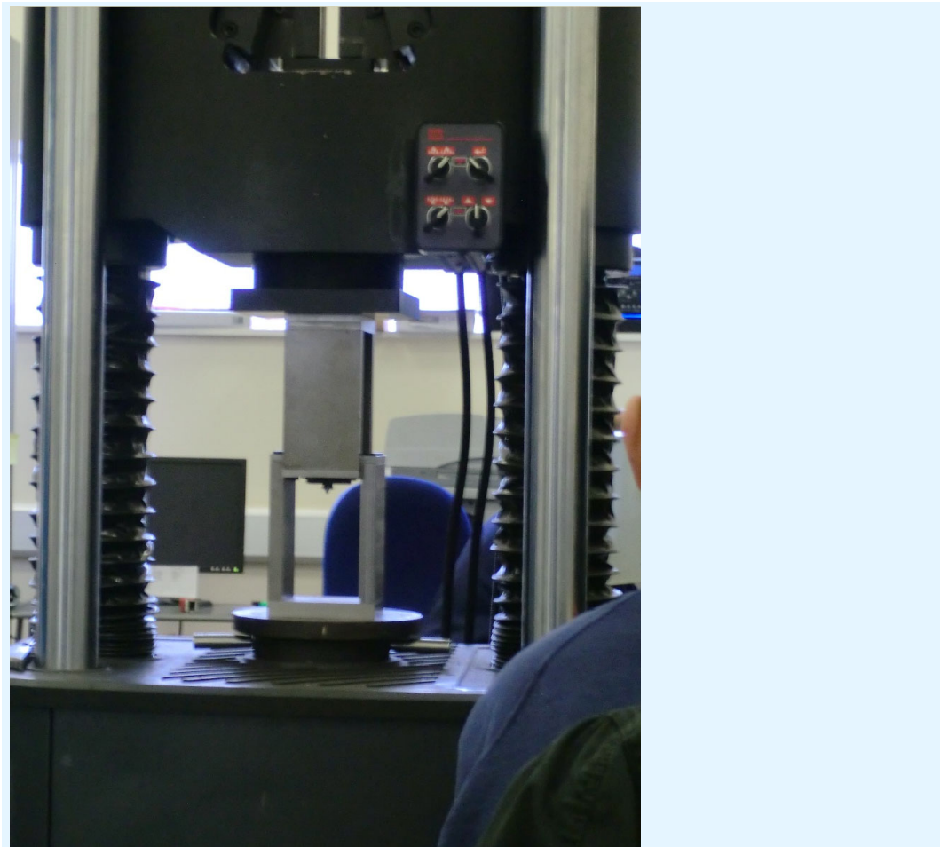
Figure 2.1 Tension test arrangement
