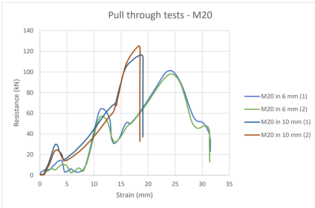
Figure A.9 M20 pull-through tests
