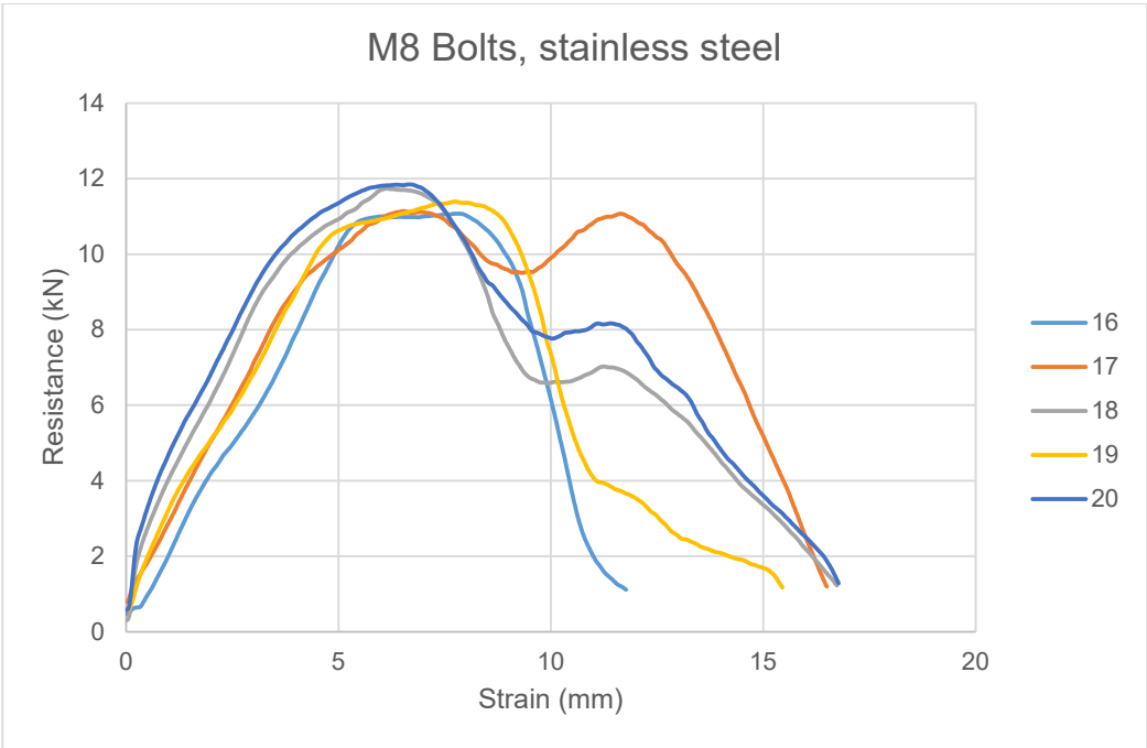
Figure A.6 M8 stainless steel test results
