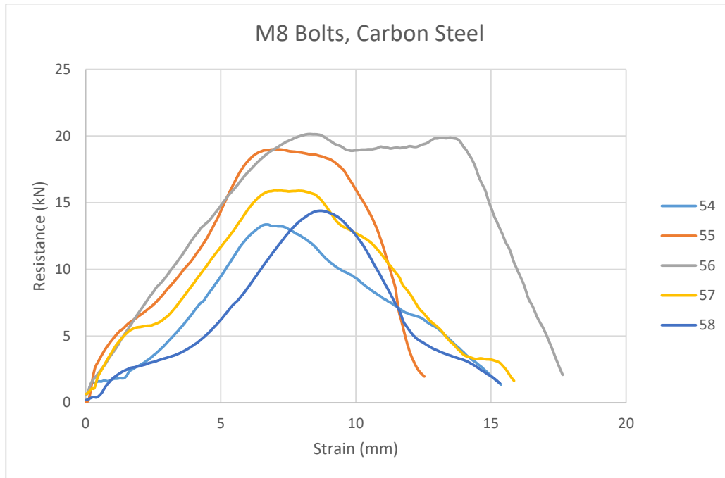
Figure A.1 M8 carbon steel test results
