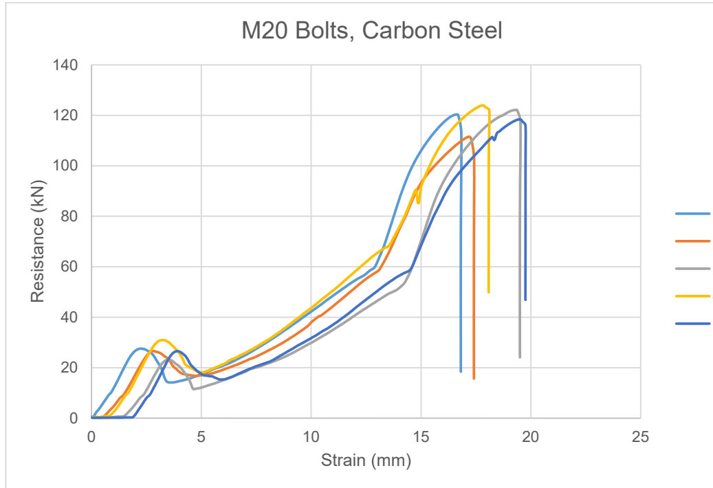
Figure A.5 M20 carbon steel test results
