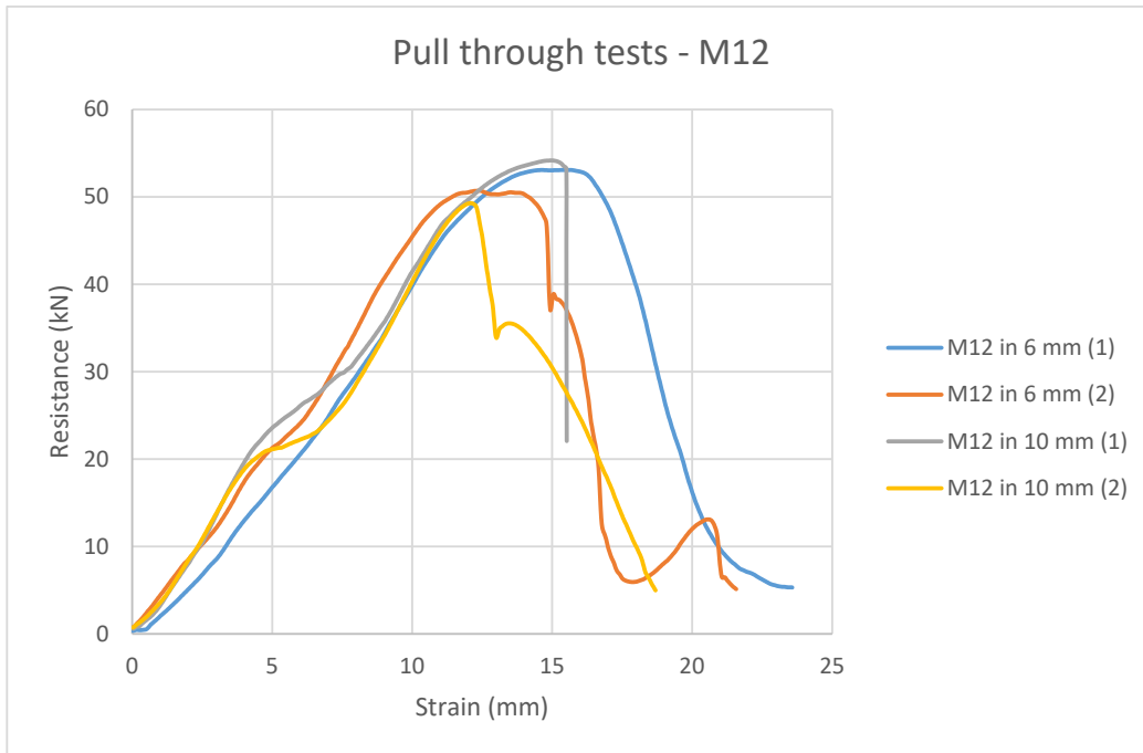
Figure A.8 M12 pull-through tests
