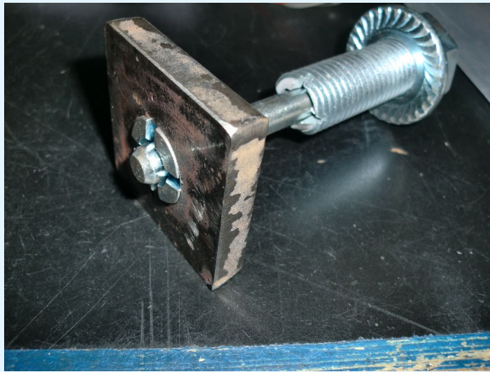
Figure 2.2 Completed tension test; fracture
