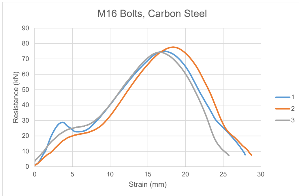
Figure A.4 M16 carbon steel test results
