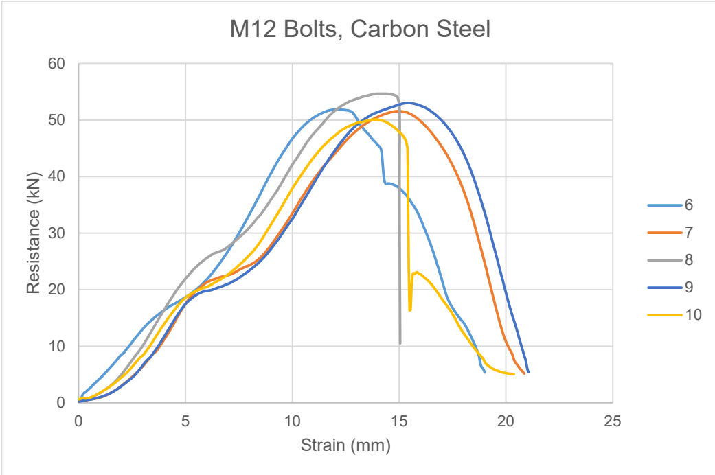
Figure A.3 M12 carbon steel test results
