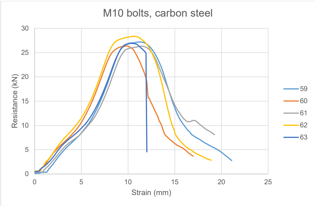
Figure A.2 M10 carbon steel test results
